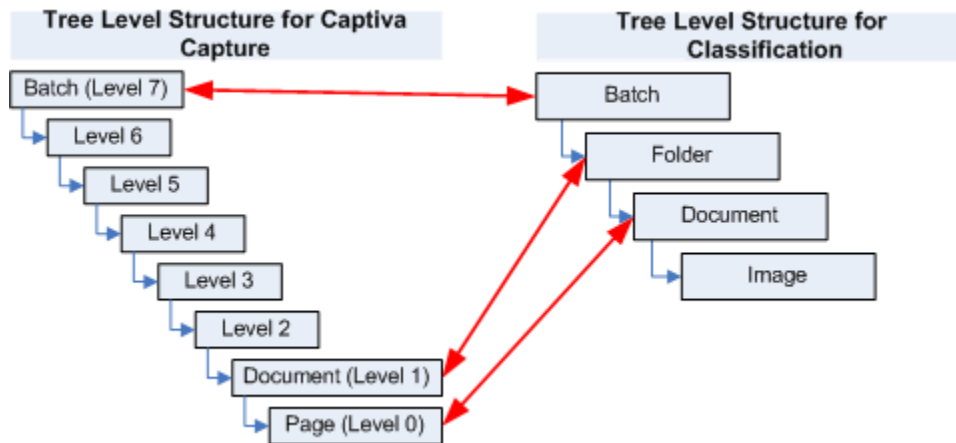
Figure 3-3: Recognition levels mapping
