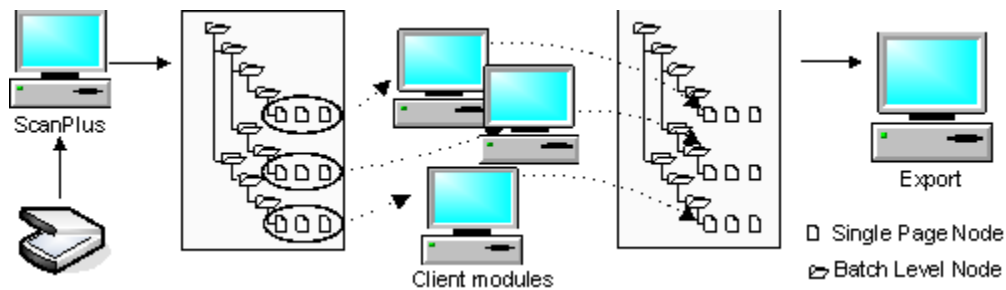
Figure 3-1: Batch tree processing
