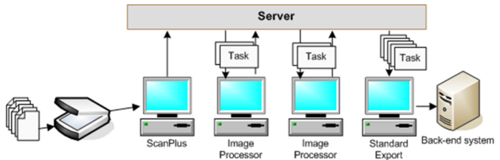
Figure 3-2: Information process
