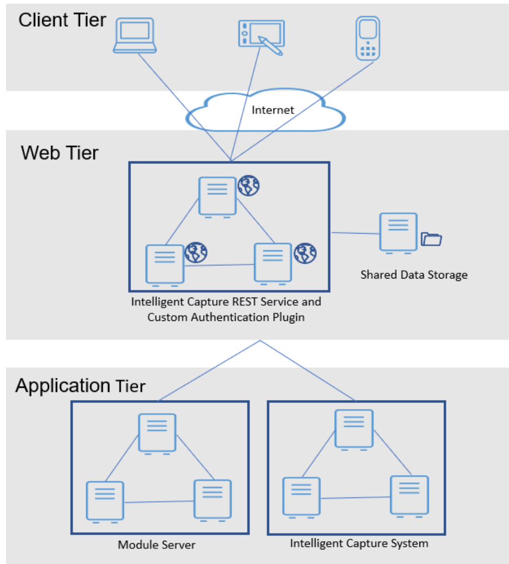
Figure 2-1: Intelligent Capture REST Services architecture
